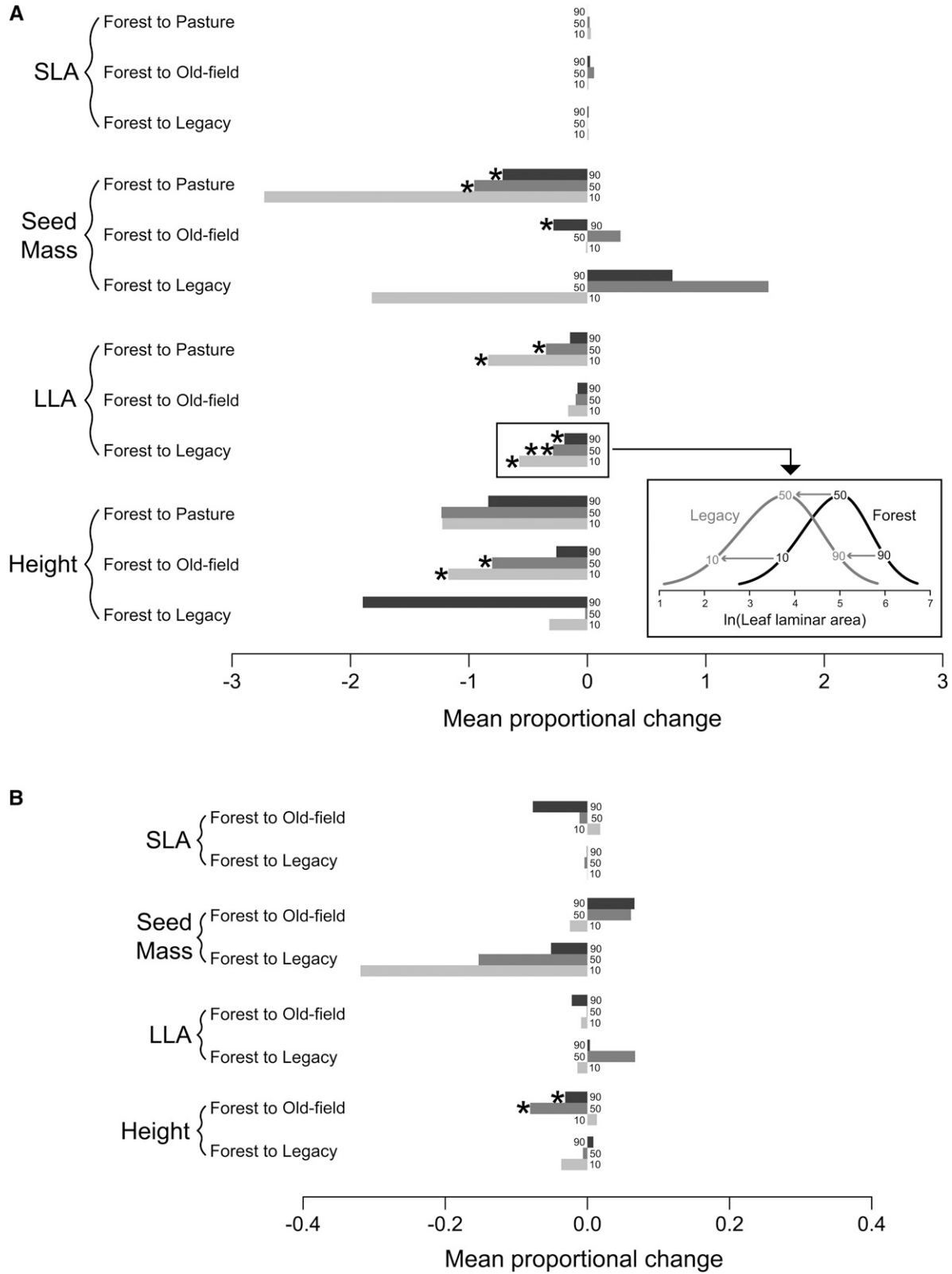
Fig. 2. Changes in the distributions of continuous traits (all ln-transformed) associated with the conversion of natural forest to other land-uses for (A) understory and (B) tree stratum. For each land-use conversion category, bars indicate the proportional change in the 10th, 50th, and 90th percentiles (averaged over the relevant studies). See inset in (A) to assist interpretation. Asterisks indicate significant changes as determined using paired two-tailed Wilcoxon sign rank tests (refer to methods and Appendix 1 for statistical details). Significant changes are generally those that are consistent (i.e., in the same direction) across all studies.
