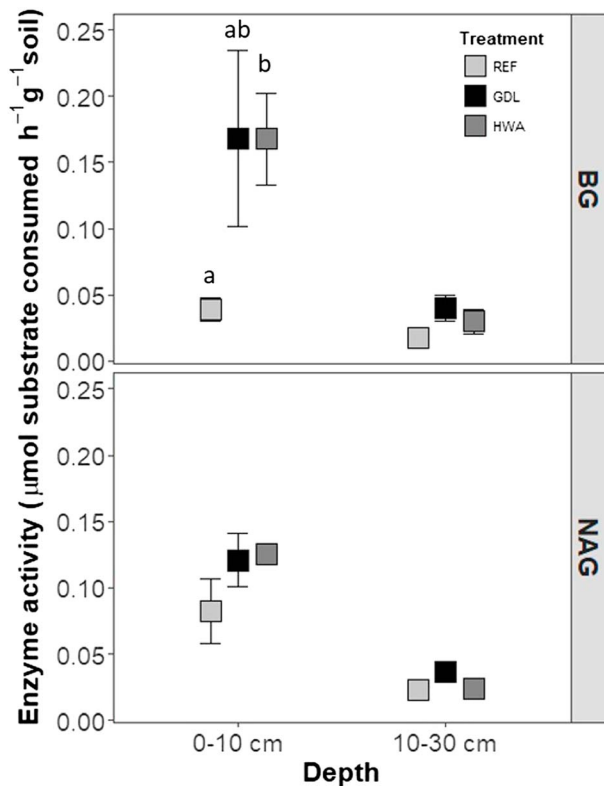
Figure 5. Activities ( \mu\text{mol substrate consumed} \cdot \text{hr}^{-1} \cdot \text{g}^{-1} \text{ soil} ; mean \pm SE) of \beta -glucosidase (BG) and \beta -1,4-N-acetylglucosaminidase (NAG) in surface (0–10 cm) and subsurface (10–30 cm) mineral soils collected in August 2014 (8 years posttreatment). GDL = girdled plots, HWA = plots infested by hemlock woolly adelgid; REF = reference plots with <3\% hemlock trees. Means with different letters indicate statistically significant differences at \alpha = 0.05 (Tukey's HSD for multiple comparisons).
